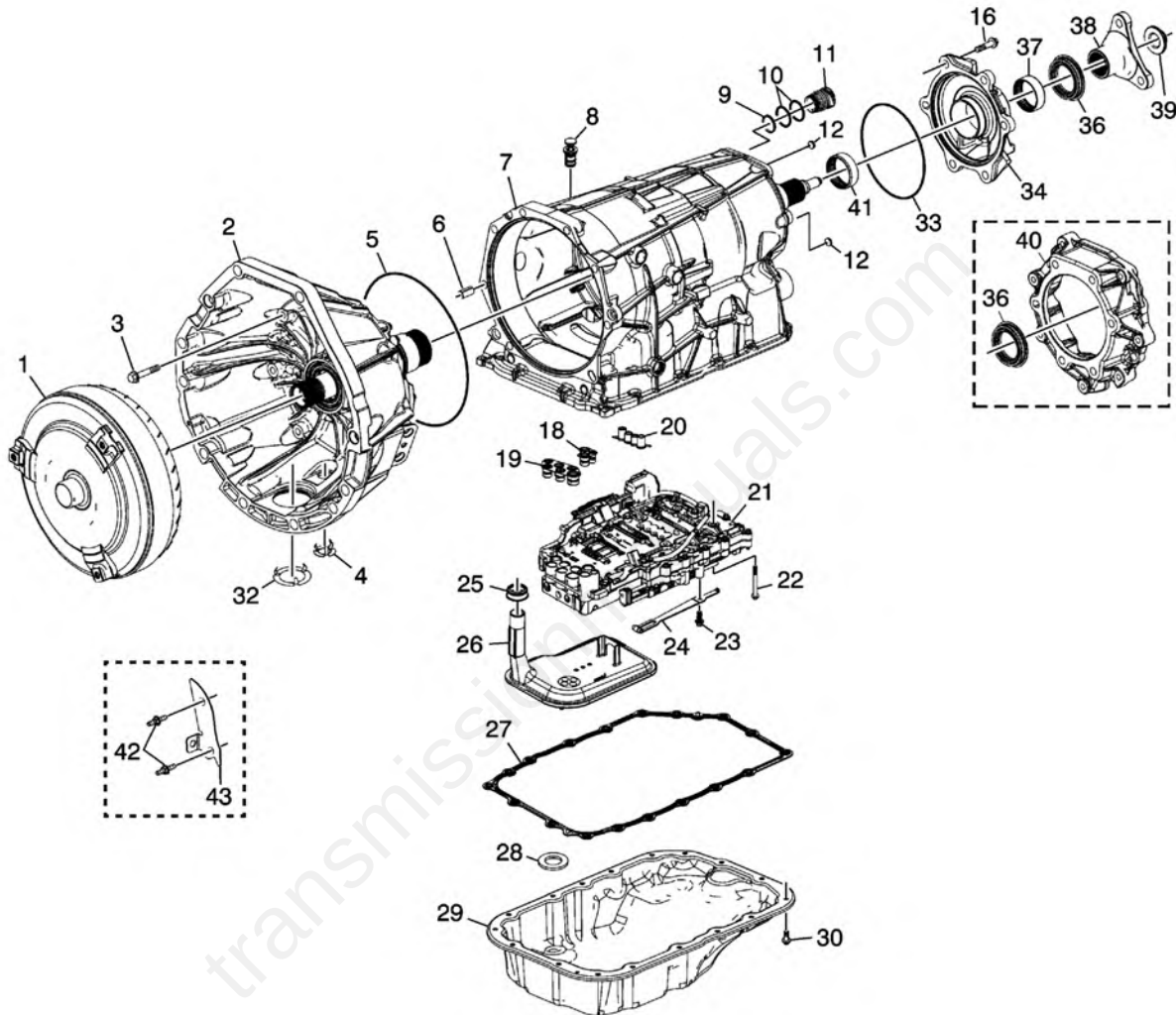
Fig. 1: Case and Associated Parts
